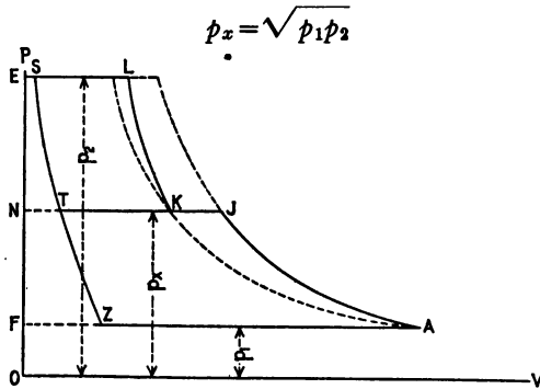
FIG. 64.—Effect of clearance on receiver pressure.
